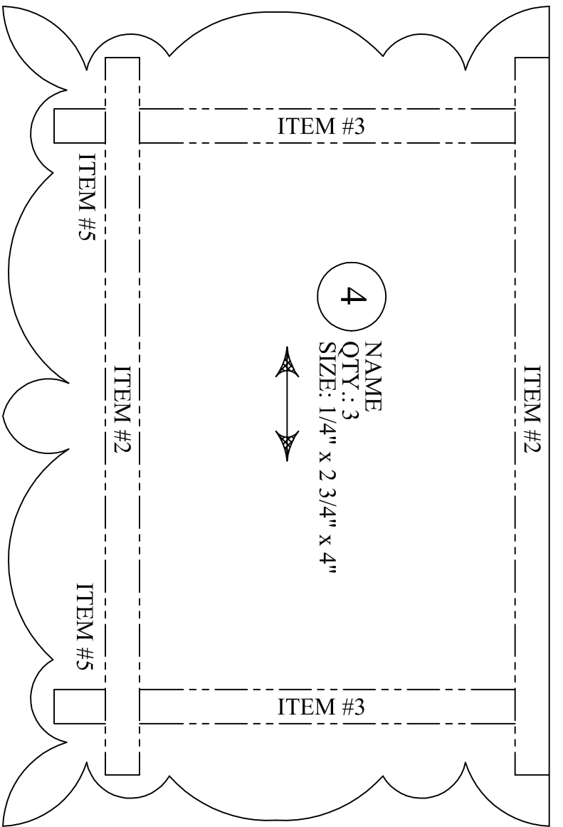
VIEW SHOWING BASE CROSS SECTION
